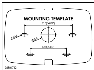
Mounting Template
